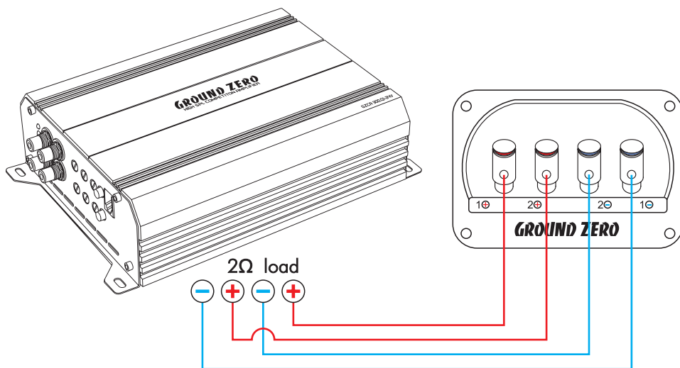
Stereo wiring @ 2Ω load pro channel
