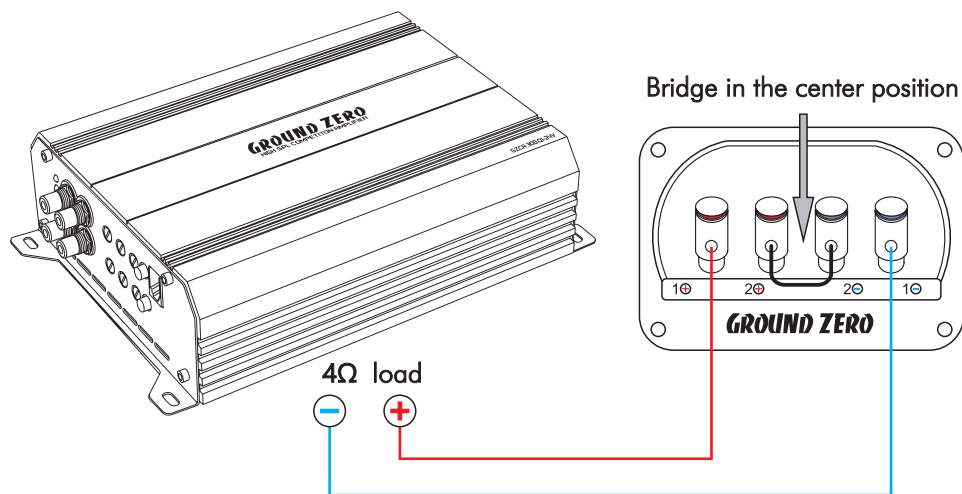
Serial wiring with one mono full range amplifier @ 4Ω load
